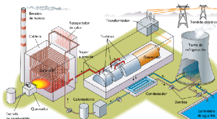
Figura 1.4. Central Termoelectrica
