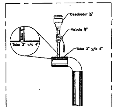
DETALLE "5"
