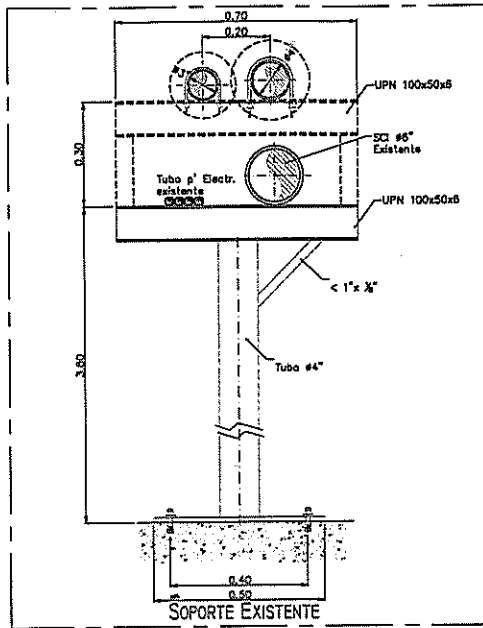
DETALLE "4"
