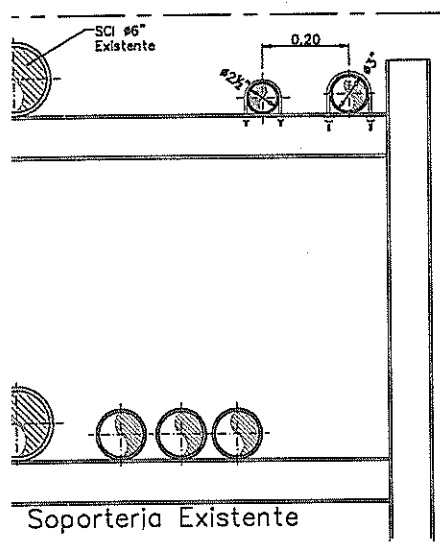
DETALLE "10"
