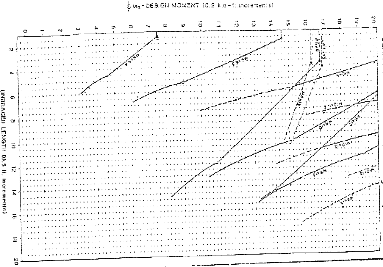
BEAM DESIGN MOMENTS ( \phi = 0.9 , C_D = 1 , F_y = 36 ksi)
