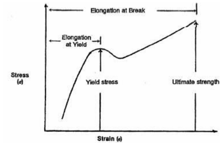
(a) Plot of results of tensile test (stress-strain curve)
