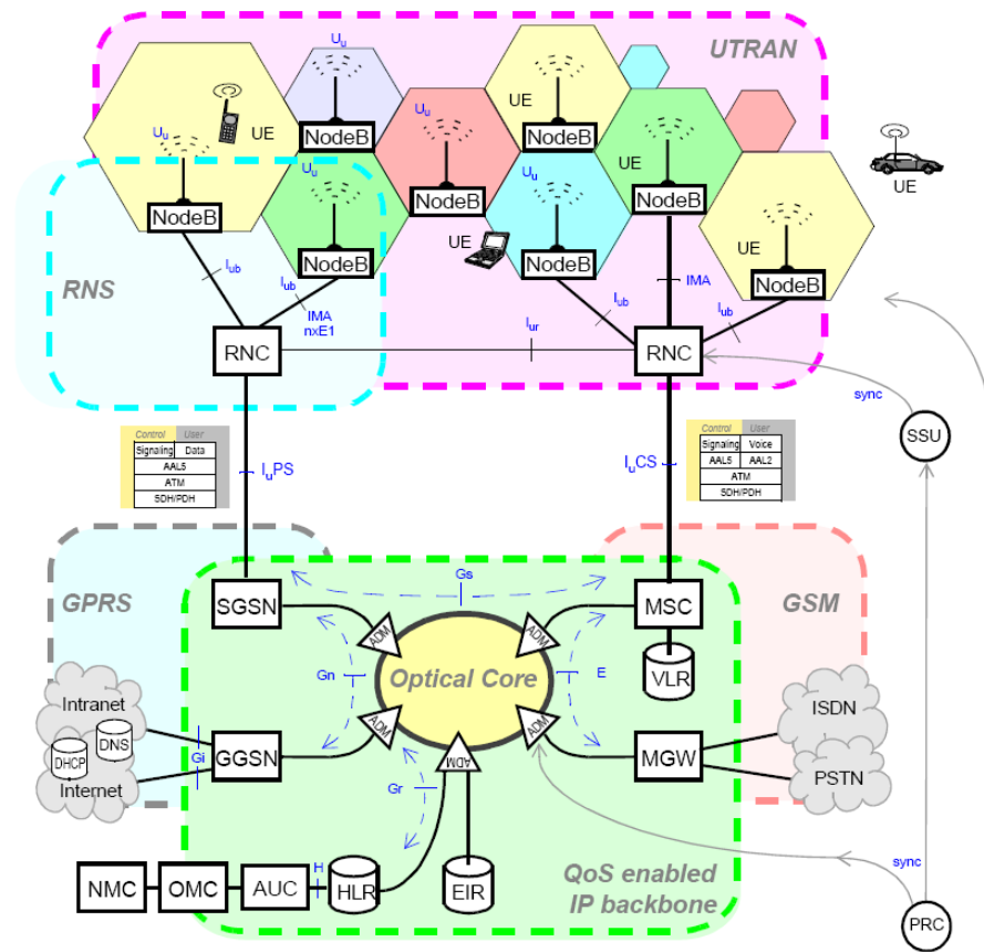
Figura 1.1: Arquitectura UMTS. [1]
