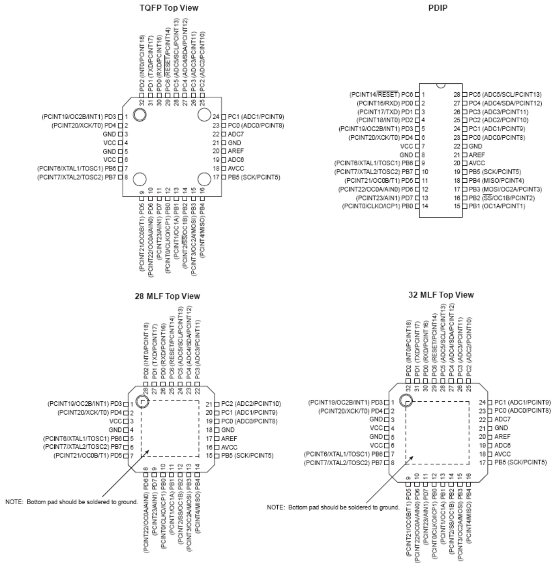
Figure 1-1. Pinout ATmega48PA/88PA/168PA/328P
