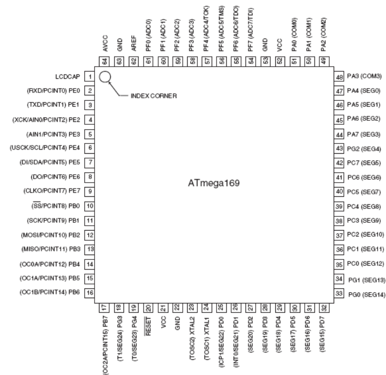
Figure 1. Pinout ATmega169
