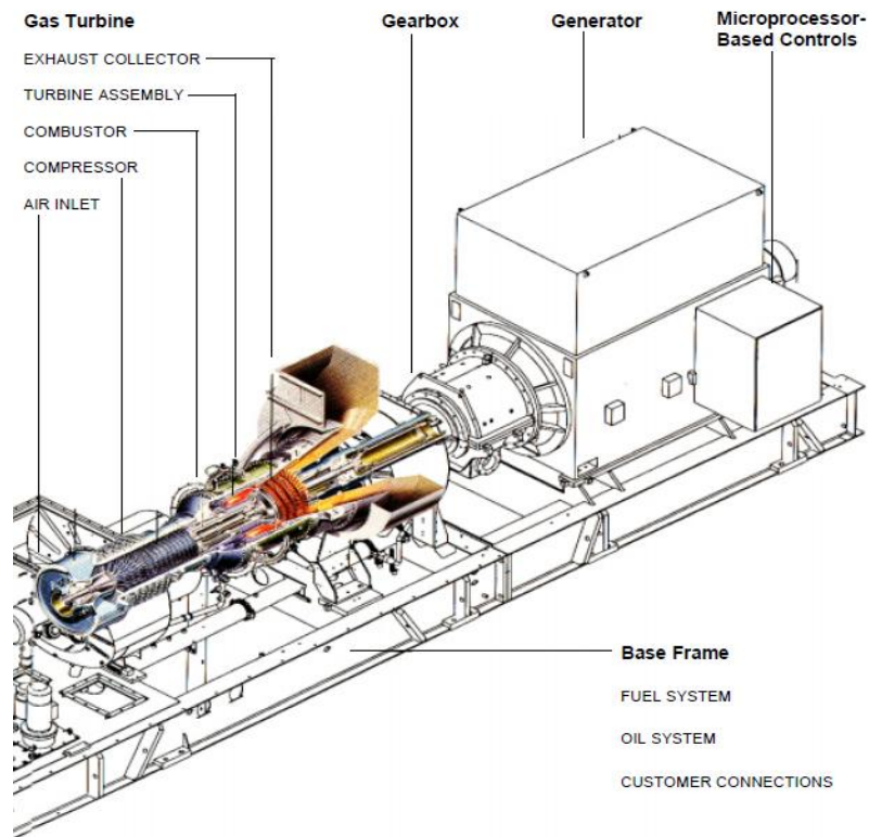
FIGURA 1.4 PARTES DE TURBINA A GAS – SOLAR TURBINES
