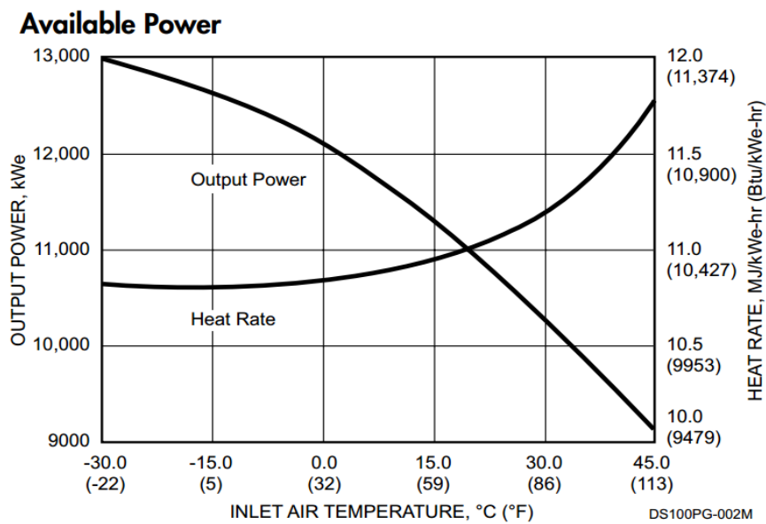
FIGURA 2.4. PERFORMANCE DATA – TURBINA AVON
