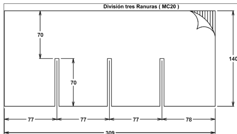
FIGURA 2. 27 DIVISION TRES RANURA
