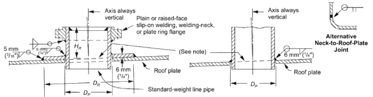
NOZZLE WITH REINFORCING PLATE
