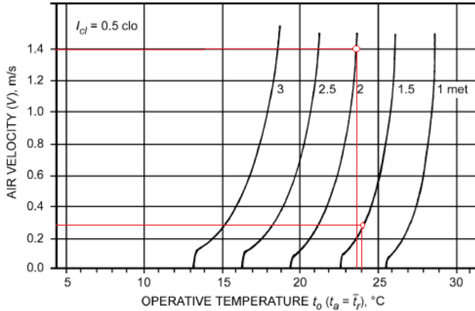
Fig. 11 Air Velocities and Operative Temperatures at 50% rh Necessary for Comfort ( PMV = 0 ) of Persons in Summer Clothing at Various Levels of Activity
