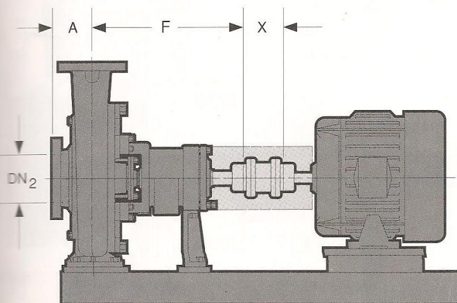
DIMENSIONS—METRIC (mm)
