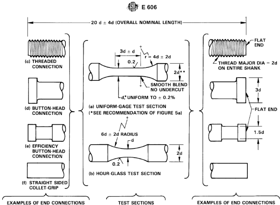
FIG. 1 Recommended Low-Cycle Fatigue Specimens
