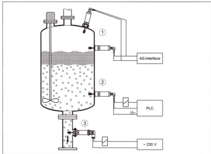
Example 1): Overflow protection or top level detection Example 2): Lower level detection or dry running protection Example 3): Dry running protection for pump
