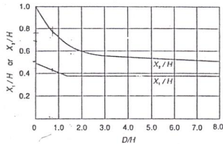
Figure E-3—Centroids of Seismic Forces
