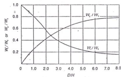
Figure E-2—Effective Masses
