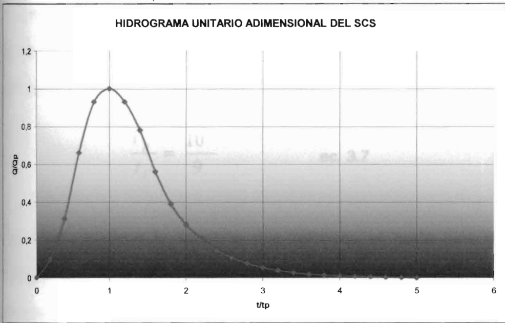
Figura 3.4.- Hidrograma Unitario Adimensional del Soil Conservation Service, SCS
