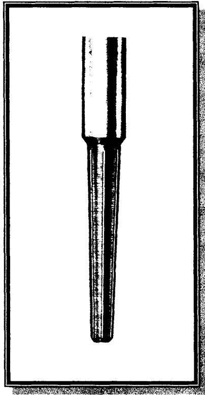
Figura 6. "Taper Tap", fuente : Bowen Fishing tools Technical Manual No.2800.
