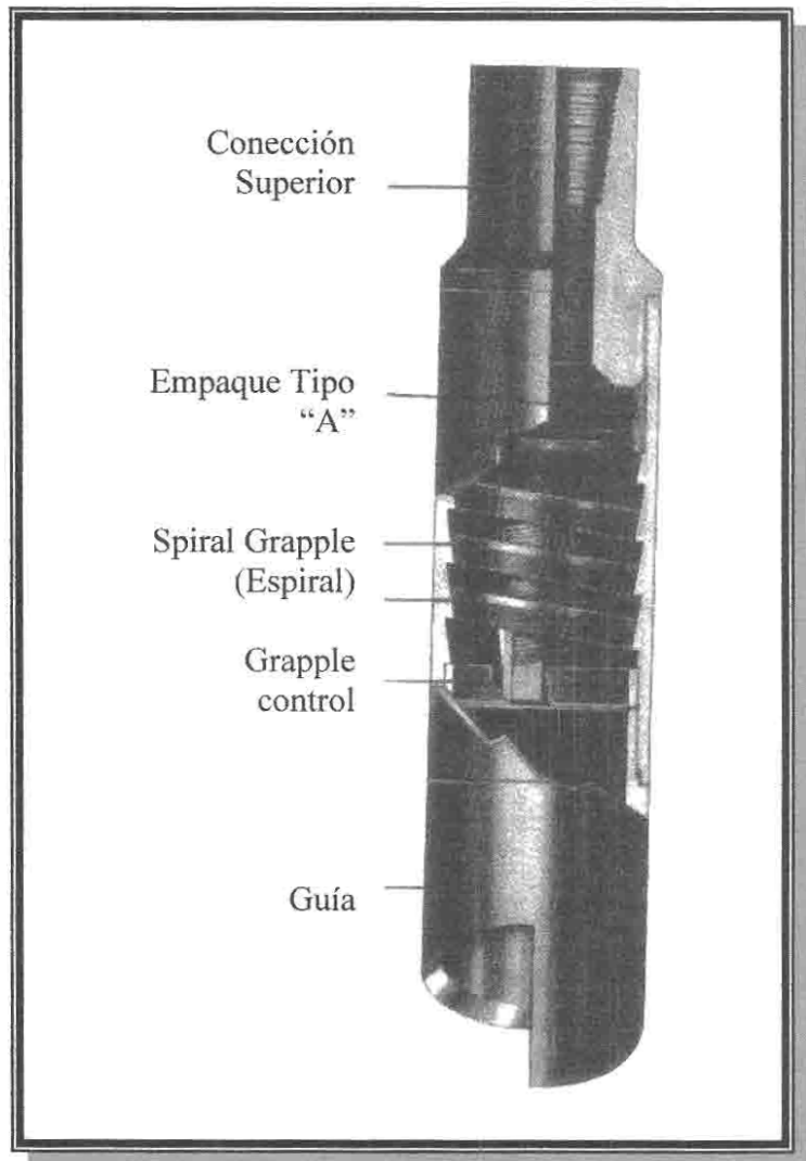
Figura 11." Overshot" con "Spiral Grapple", fuente: Bowen Fishing tools Technical Manual No.1150.
