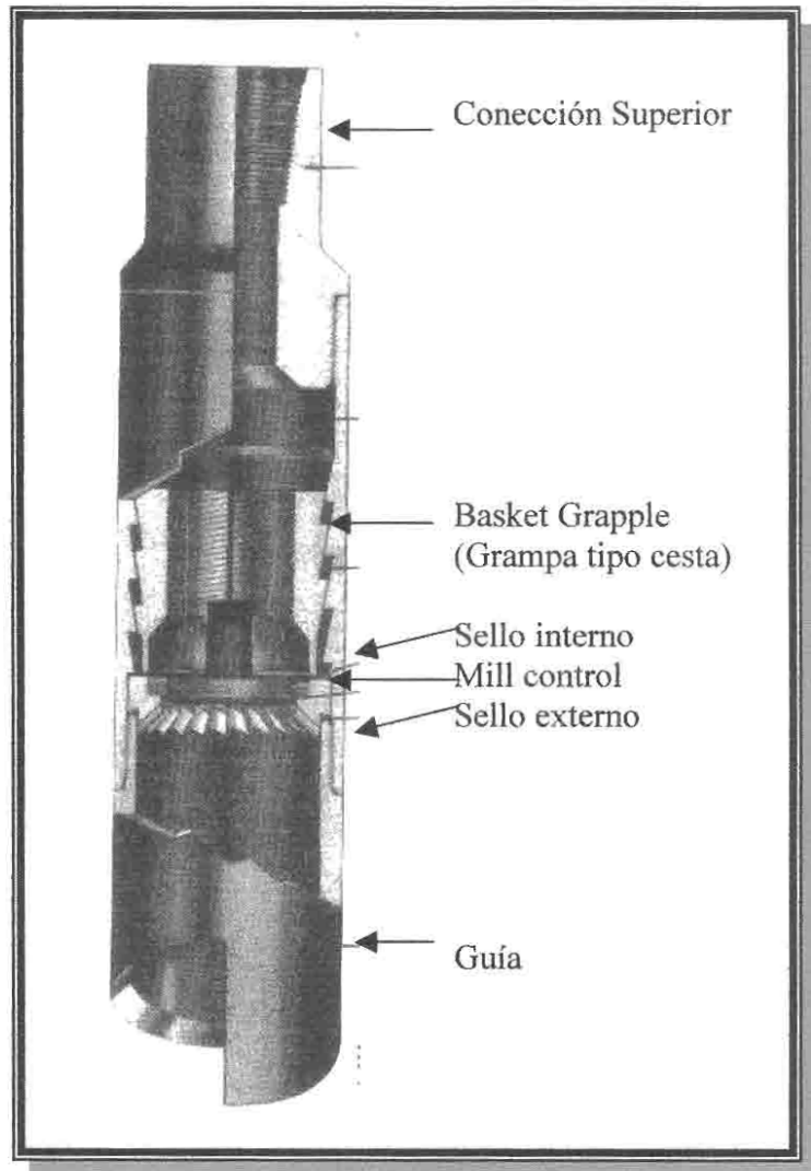
Figura 10. "Overshot" con "Basket Grapple", fuente: Bowen Fishing tools Technical Manual No.1150.
