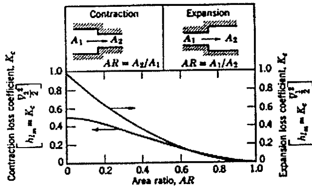
Fig. 8.16 Loss coefficients for flow through sudden area changes (Ref. 5).
