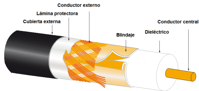
Figura 4.15 Cable coaxial [44]
