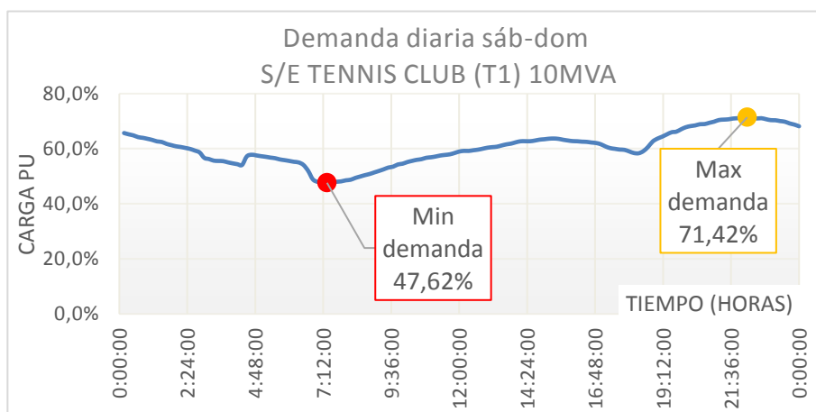
Figura 2.3: Demanda diaria sáb-dom S/E TENNIS CLUB 10 MVA
