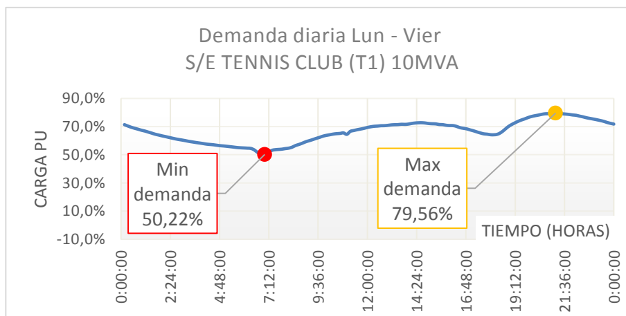
Figura 2.9: Demanda diaria lunes-viernes S/E TENNIS CLUB 10 MVA
