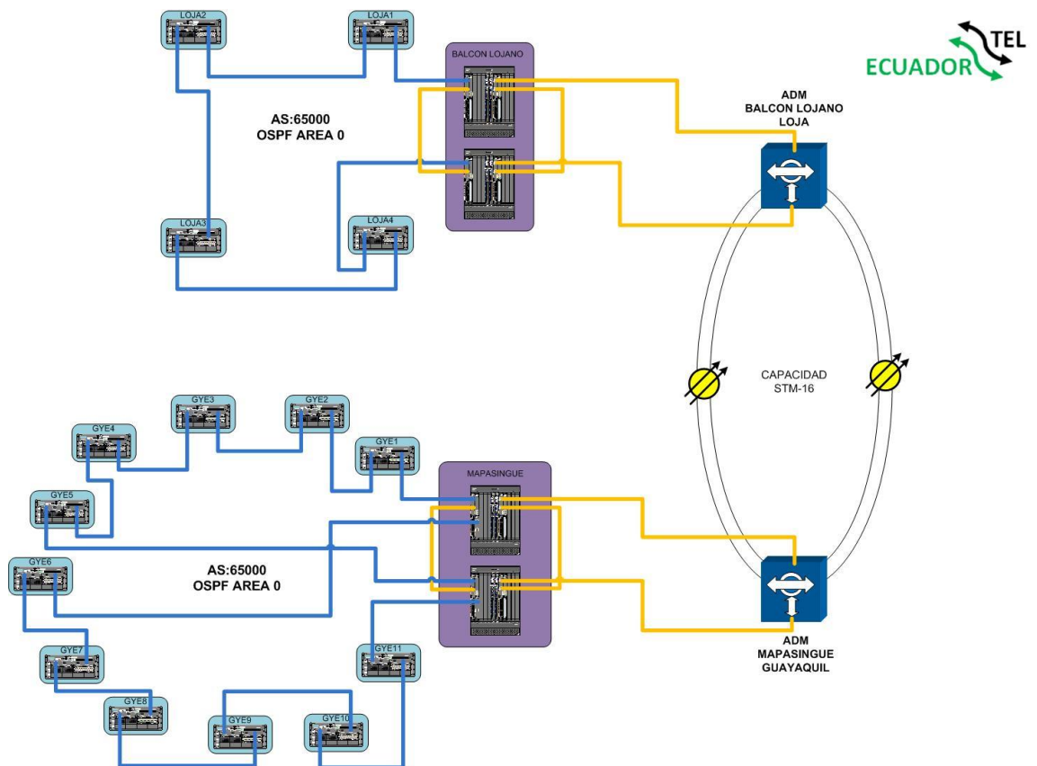
Figura 3.19 Red integrada SDH-IP/MPLS Loja – Guayaquil.
