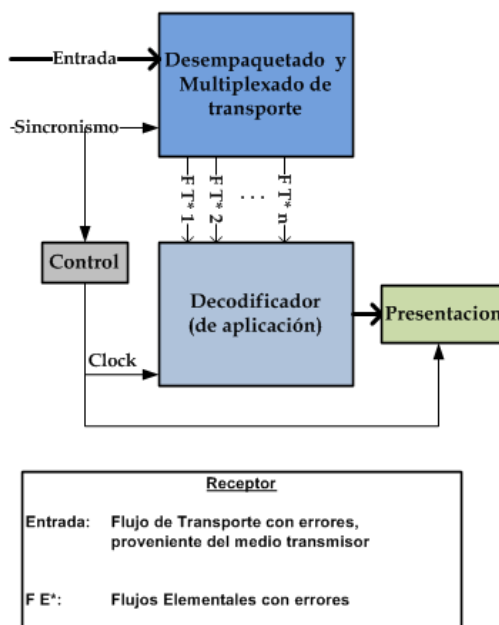
Figura 3.10 Receptor
