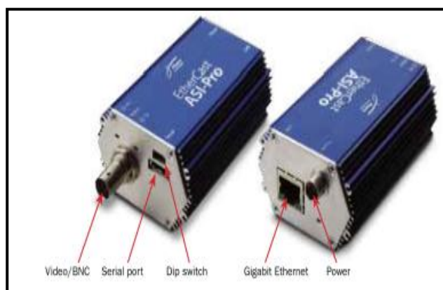
Figura 2.8 Gateway IP EtherCast ASI-Pro
