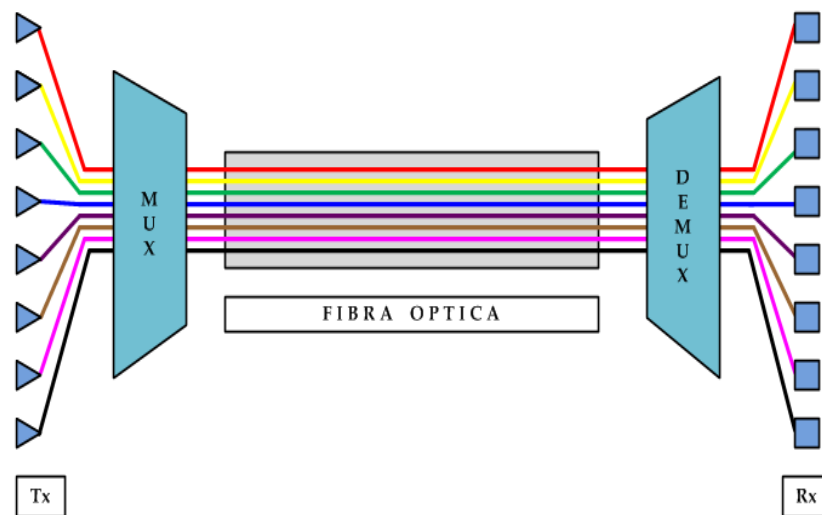
Figura 5.4 DWDM
