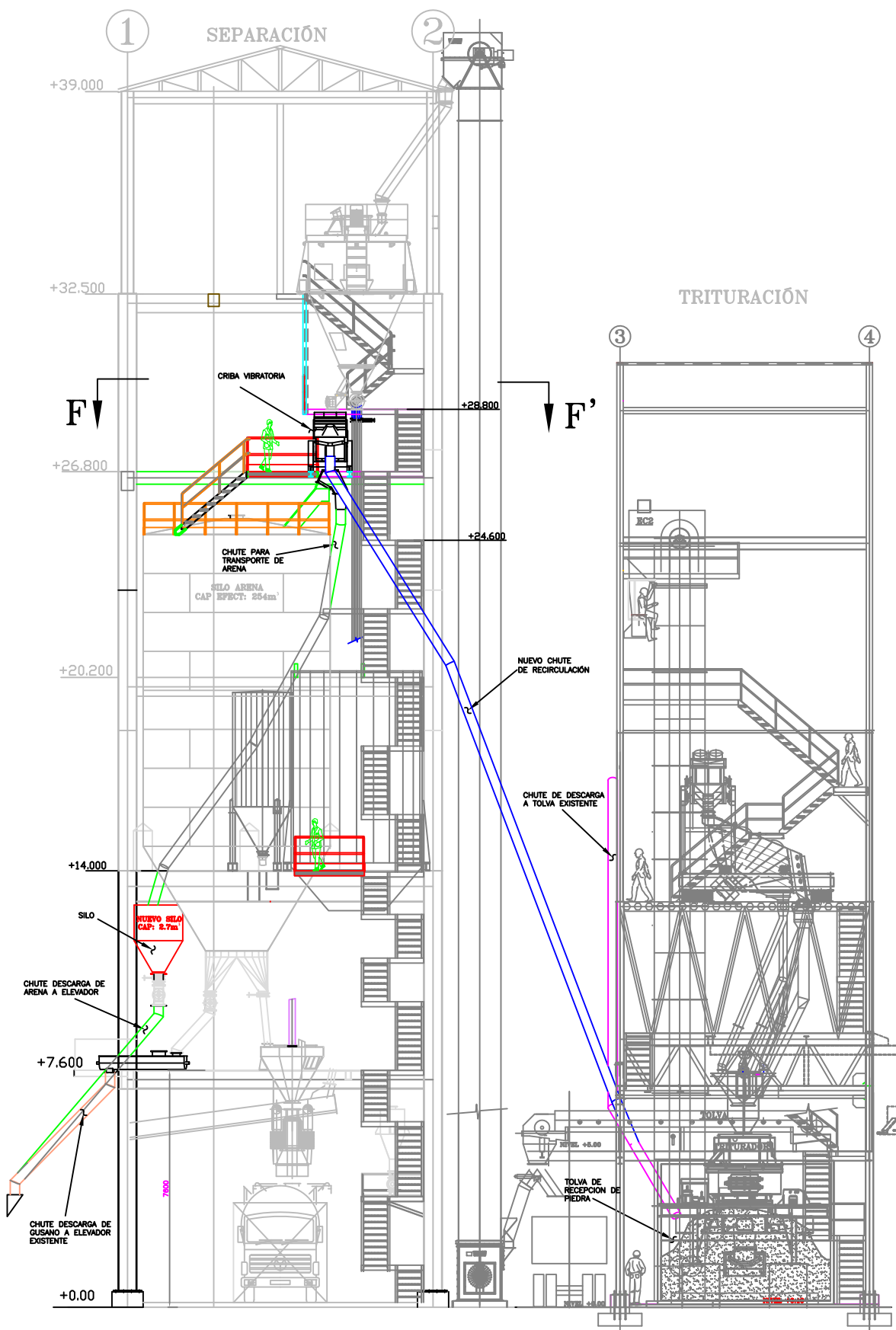
VISTA FRONTAL
