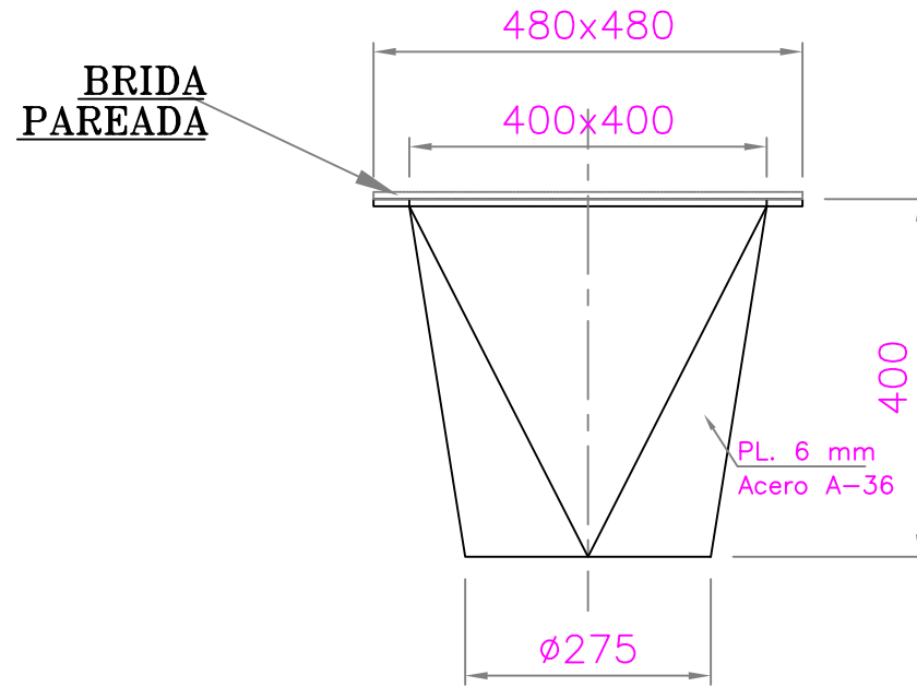
1 TRANSICION CANT: 1 ESCALA 1:10
