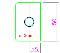
5 ESPIGO (Cant. 1u) ESCALA 1 : 1.5
