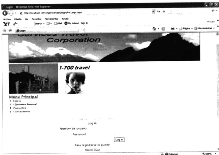
Figura 7-7: Login
