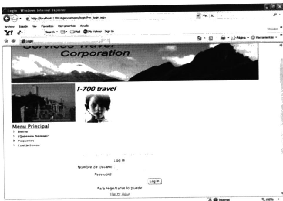
Figura 9-8: Log in.
