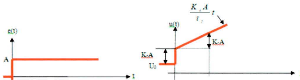
FIGURA 1.22: CONTROL PROPORCIONAL - INTEGRAL (PI)
