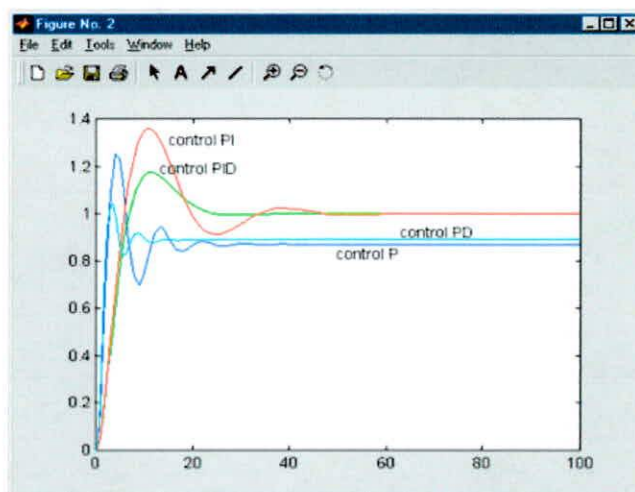
FIGURA 1.23: CONTROL PROPORCIONAL – INTEGRAL – DERIVATIVO
