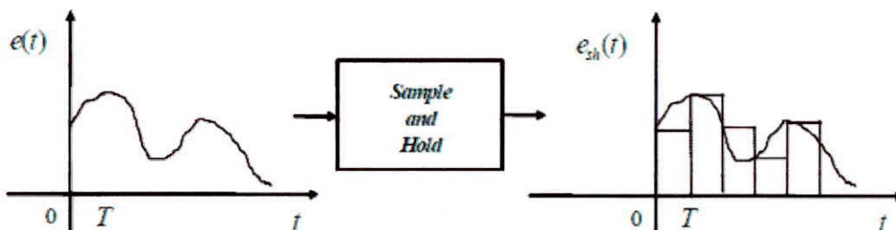
FIGURA 1.31: EFECTO SAMPLE AND HOLD
