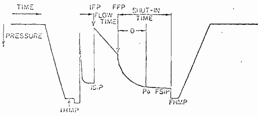
Typical DST Chart (Double Shut-in Test)
