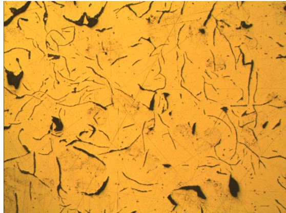
Figura 2.2 Material Base 100x Sin Ataque
