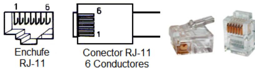
Figura 4.35 Conector RJ-11.
