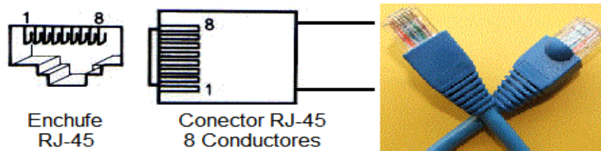
Figura 4.36 Conector RJ-45.
