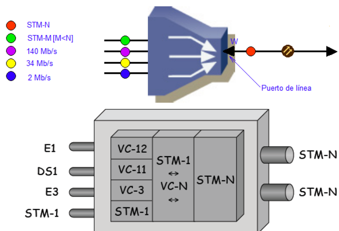
Figura 1.1 Multiplexor Terminal (TM).
