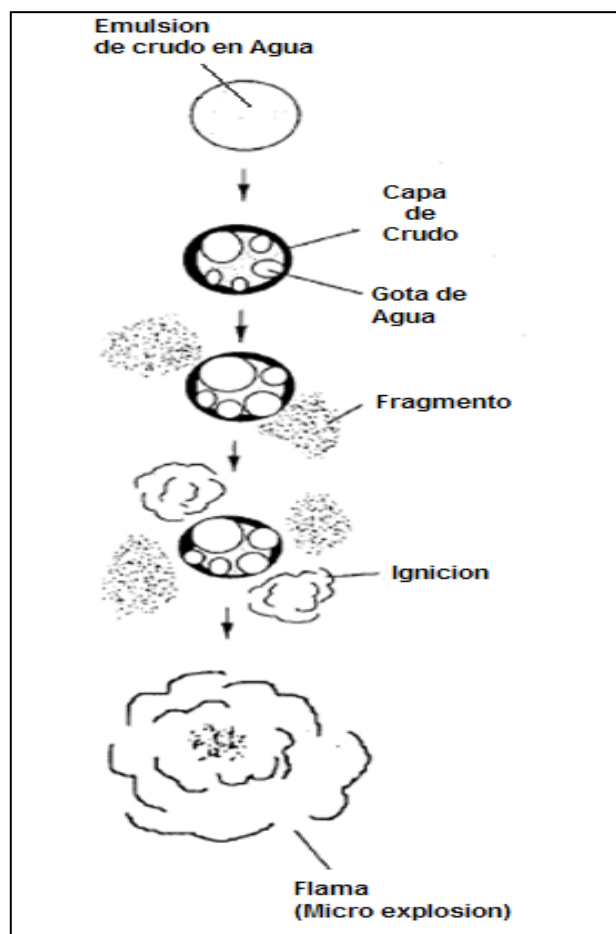
FUENTE [ Ignition and Combustion Behavior of Asphalt/Water-Emulsified Fuels, K. Namba and K. Kumuto, "JSME International Journal"] FIGURA 1.8 – PROCESO DE LA EMULSIÓN FOE.
