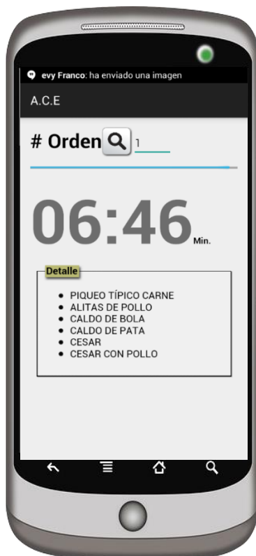
Figura 2.21: App Android
