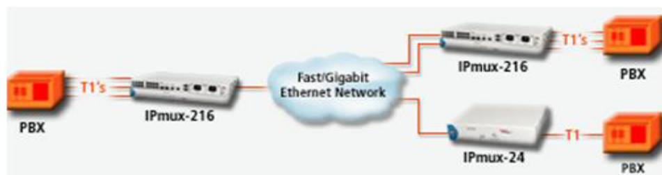
Figura 1.16 Red TDMoIP [19]
