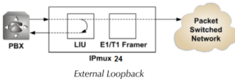
Figura 3.73 Loop External
