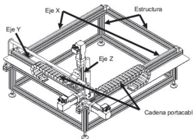
Figura 2.1: Mesa cartesiana XYZ [2].
