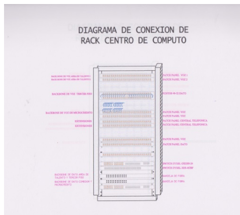
Figura a. 1 Diagrama del rack Principal
