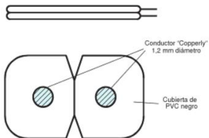
FIG.17.18 CABLE DE ACOMETIDA BIMETALICA [15]
