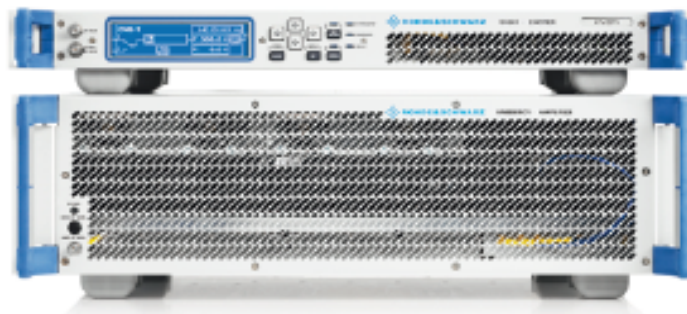
R&S®SCx8000 transmitter configured as R&S®CV0801EA with an R&S®VM8901C1 VHF amplifier and an R&S®D0801 exciter. All VHF models have only one amplifier.
