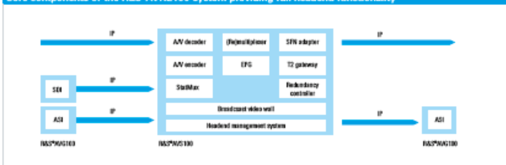
Core components of the R&S®AVHE100 system providing full headend functionality
