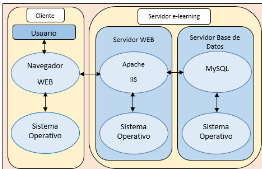
Figura 2-2: Diagrama de Despliegue de Moodle. [1]
