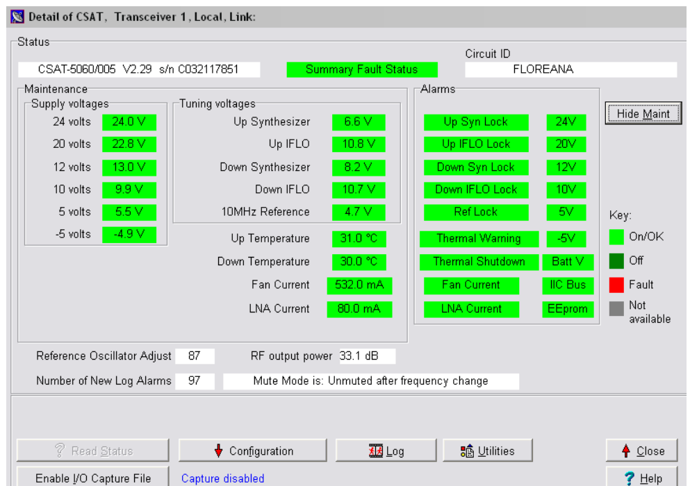
Figura 3. 12: Consumo transceptor.
