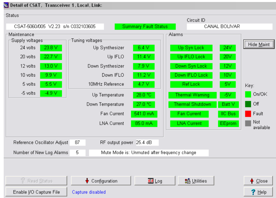
Figura 3. 16: Consumo transceptor.
