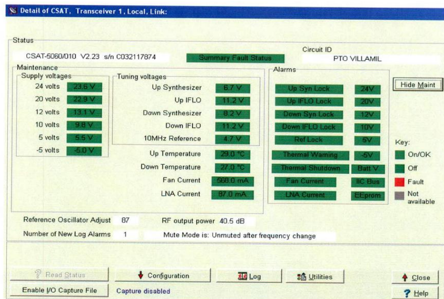
Figura 3. 15: Consumo transceptor de 10 watts.
