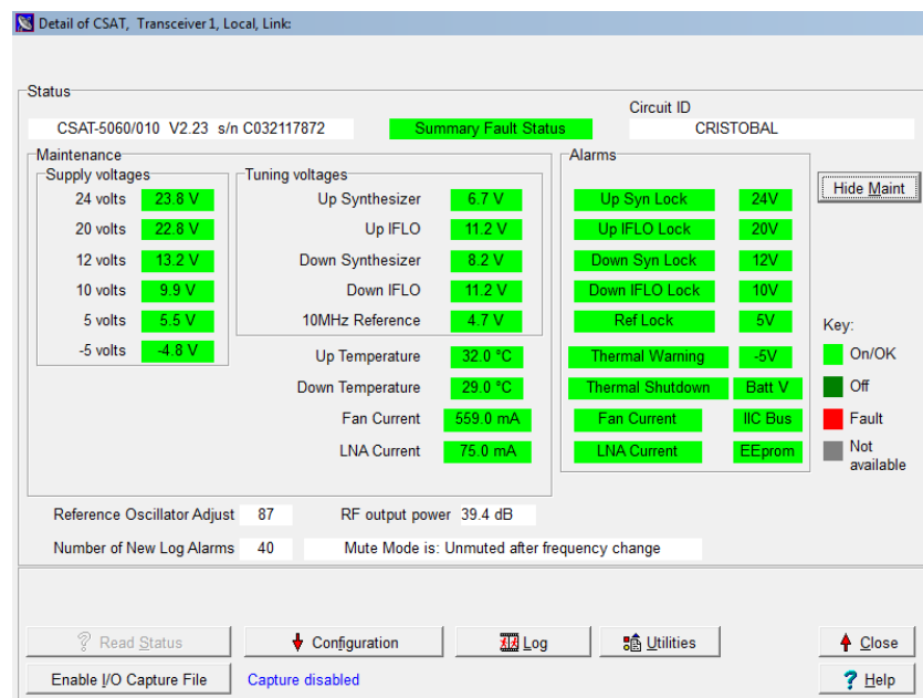
Figura 3. 9: Consumo transceptor.
