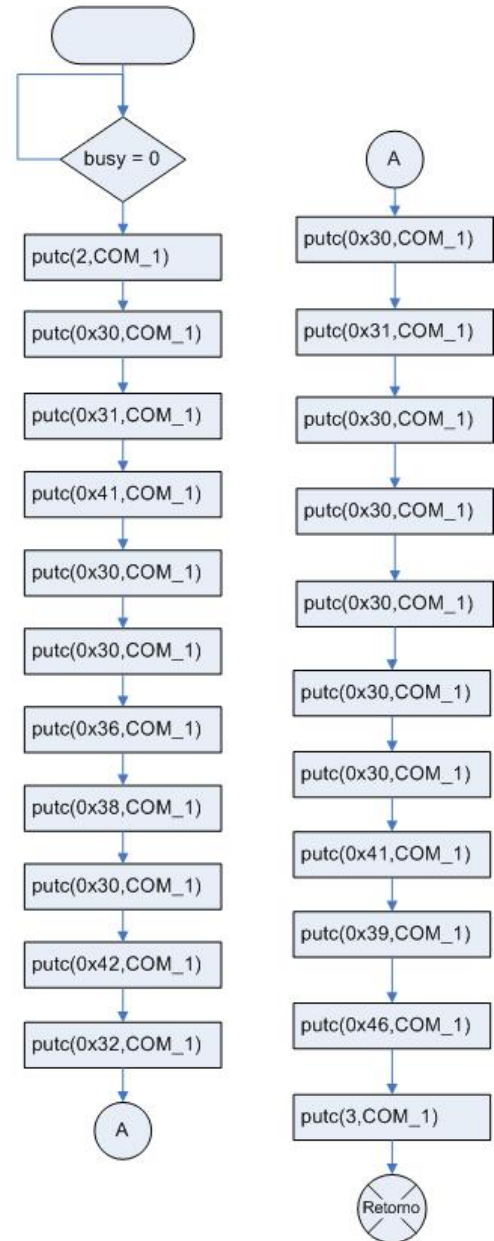
read_data_1()
