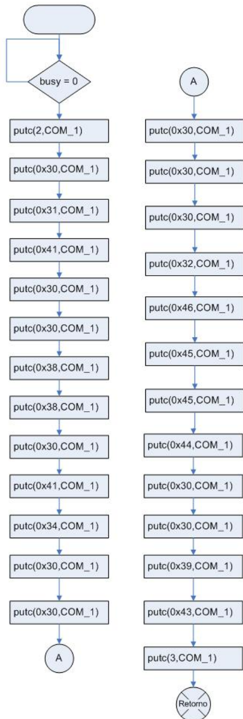
Select_file_2()
