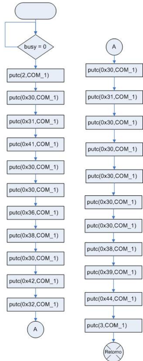
read_data_2()
