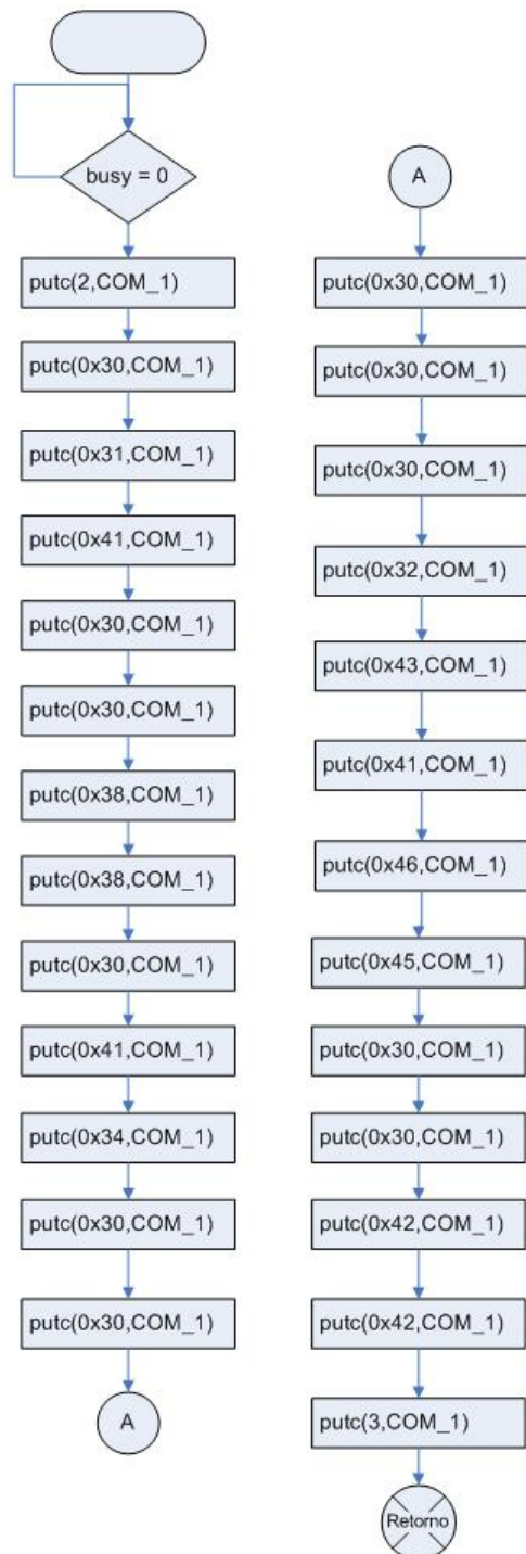
Select_file_1()
