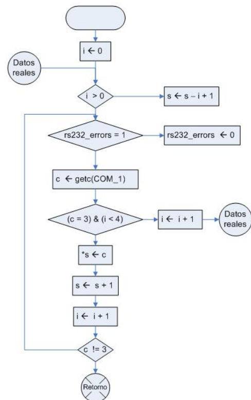
getss(char *s)
