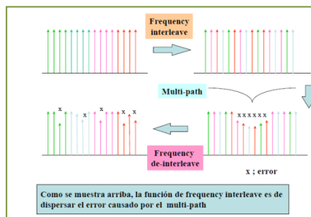
Figura 2.3.5.1.3 Efecto del Frequency Interleave [15]
