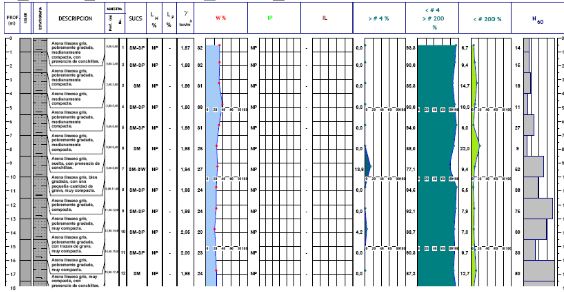
Sondeo B-132 B (1/2)
