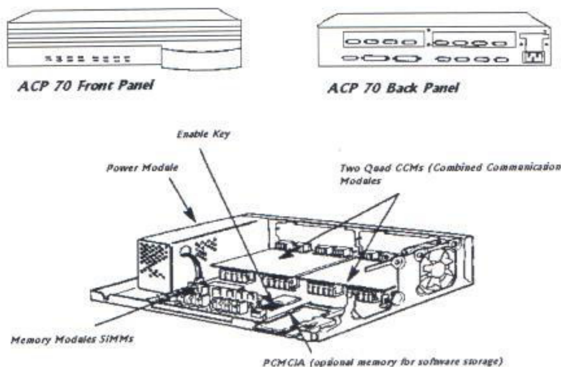
Figura 7: Chasis ACP 70
